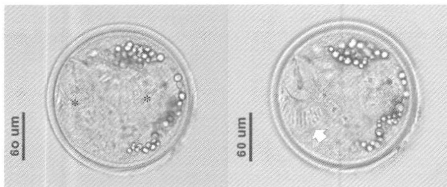
Figure 1 An isolated metacercariae of Echinostoma revolutum showing a well-developed oral and ventral sucker (asterisk) and head collar with collar spines (arrowhead).
