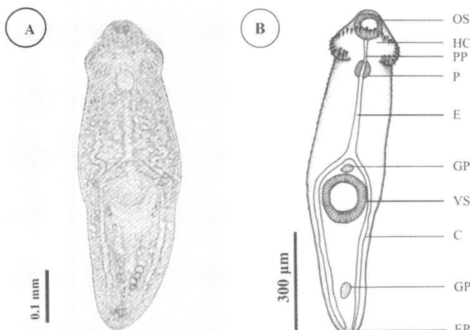
Figure 2 Illustration demonstrating excysted metacercaria of Echinostoma revolutum ; (A) Photograph of excysted metacercaria compressed under a cover slip. (B) Drawing. Abbreviations: C, Caeca; E, Esophagus; EP, Excretory pore; GP, Genital primordia; HC, Head crown; OS, Oral sucker; P, Pharynx; PP, Prepharynx; VS, Ventral sucker.
